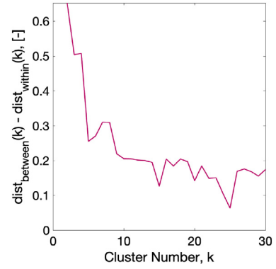
Fig. 13. Determination of optimal number of clusters, N_c , as in Eq. (8), by applying k -means clustering to P for different number of clusters k , up to k_{\max} = 30 . From this plot, N_c = 2 .
