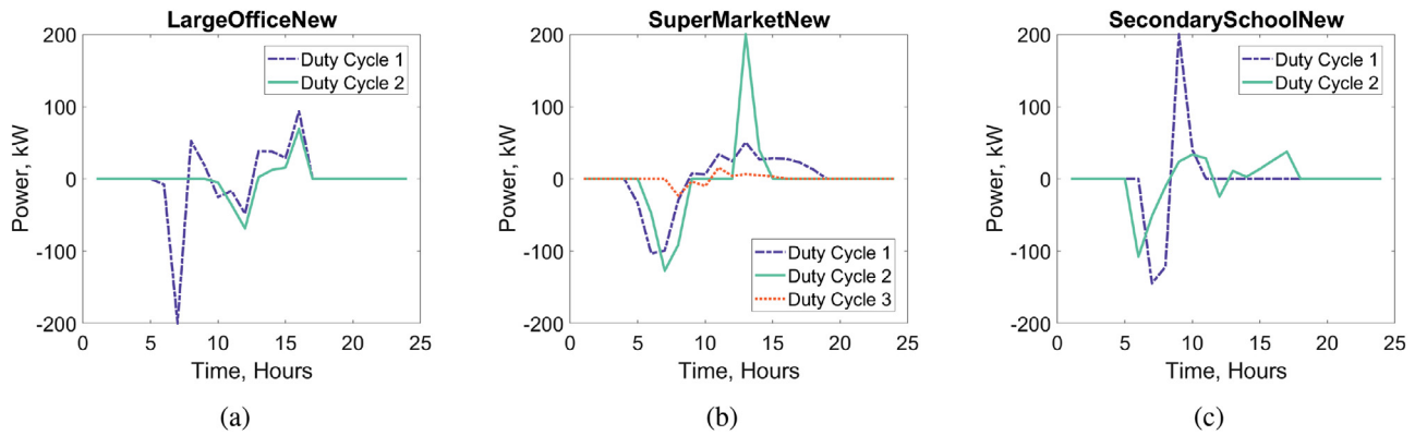
Fig. 15. Characteristic duty cycles for peak shaving dispatch on the (a) LargeOfficeNew, (b) SuperMarketNew, and (c) SecondarySchoolNew load profiles.
